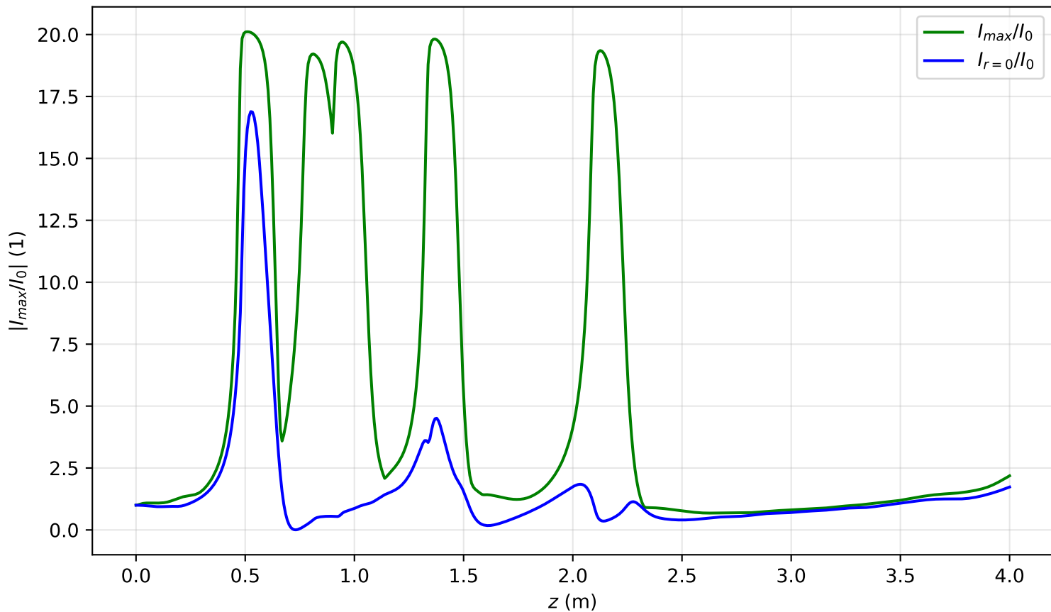
I_{max}(x = 0, y = 0, z)/I_0 , P_{in}=5.5P_{cr} , noisy input, artificial time
